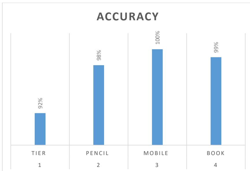
Fig.2. Accuracy.
