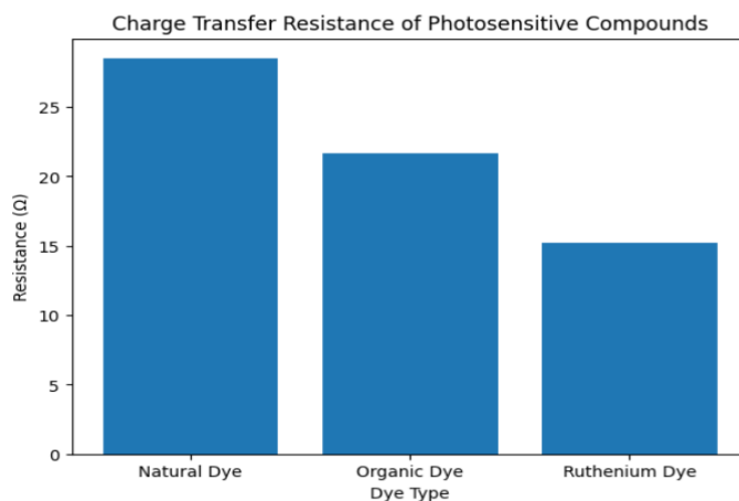
Figure 4 Charge Transfer Resistance of Compounds
