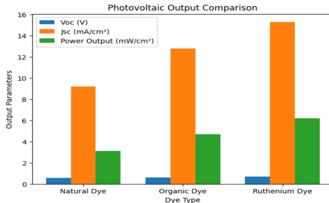
Figure 3 Photovoltaic Output Comparison
