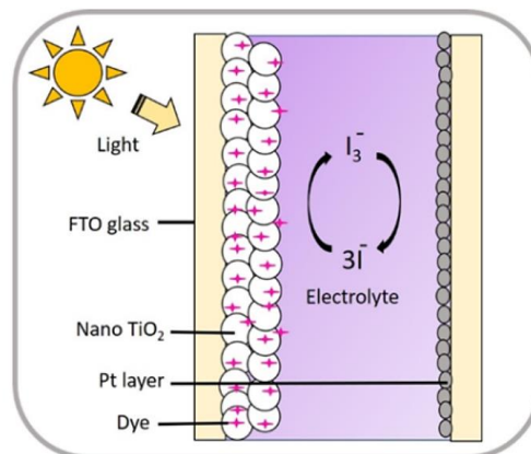
Figure 1 Components of dye-sensitized solar cells (DSSCs)
