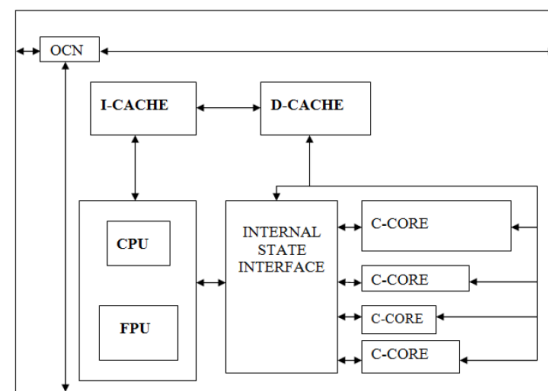
Figure 4.: Architecture of Each Tile.
